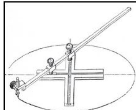
Ellipsographs
